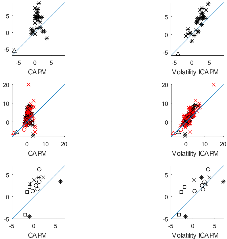
Figure 4: Each diagram plots sample against predicted average excess returns. Test assets in the top row are the 25 ME- and BE/ME-sorted portfolios (asterisks), plus the t-bill return (triangle); in the middle row, both unscaled (black) and scaled by EVAR (red) versions of the 25 ME- and BE/ME-sorted portfolios (asterisks), six risk-sorted portfolios (circles), 18 characteristic- and risk-sorted portfolios (crosses), and t-bill return (triangles); and, in the bottom row, the three fama-French factors and the Coval-Shumway straddle (asterisks), interest-rate-sorted portfolios (circles), the two risk bond factors of Fama and French (crosses), and three variance forwards (squares). Predicted values are from Table 4 (top row) and Table 5 (middle row) for 1963:3-2011:4 and from Table 6 (bottom row) for 1998:1-2011:4. From left to right, the models tested are the CAPM and the three-factor ICAPM.
